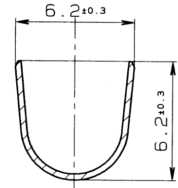
SEC. B-B
