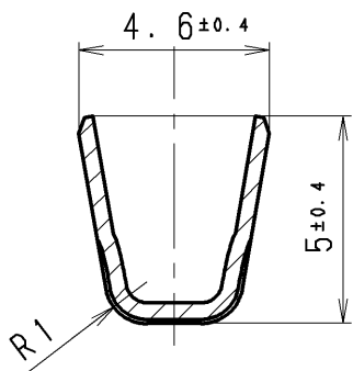
SEC. B-B
