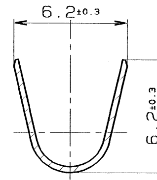
SEC. B-B
