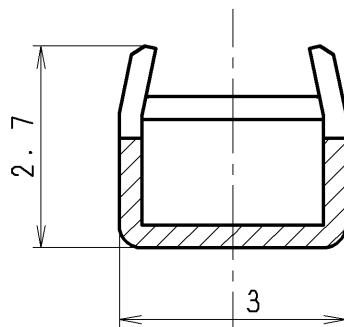
SEC. C-C (10/1)
