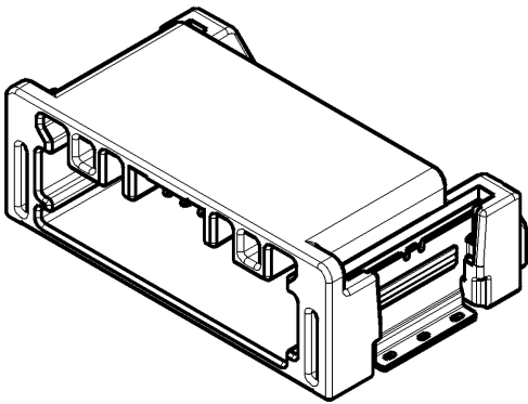
ISOMERIC VIEW
