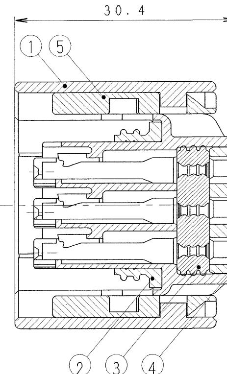
SECTION AA
