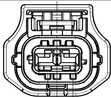
CODING-C PART NO.6189-7530
