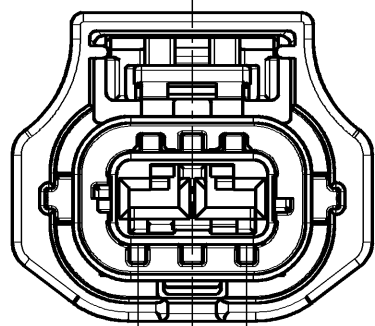
CODING-C PART NO.6189-7530
