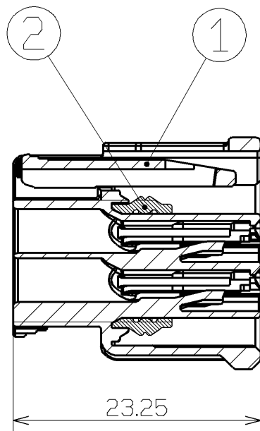
SECTION AA
