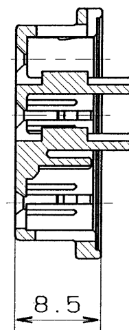
SECTION AA
