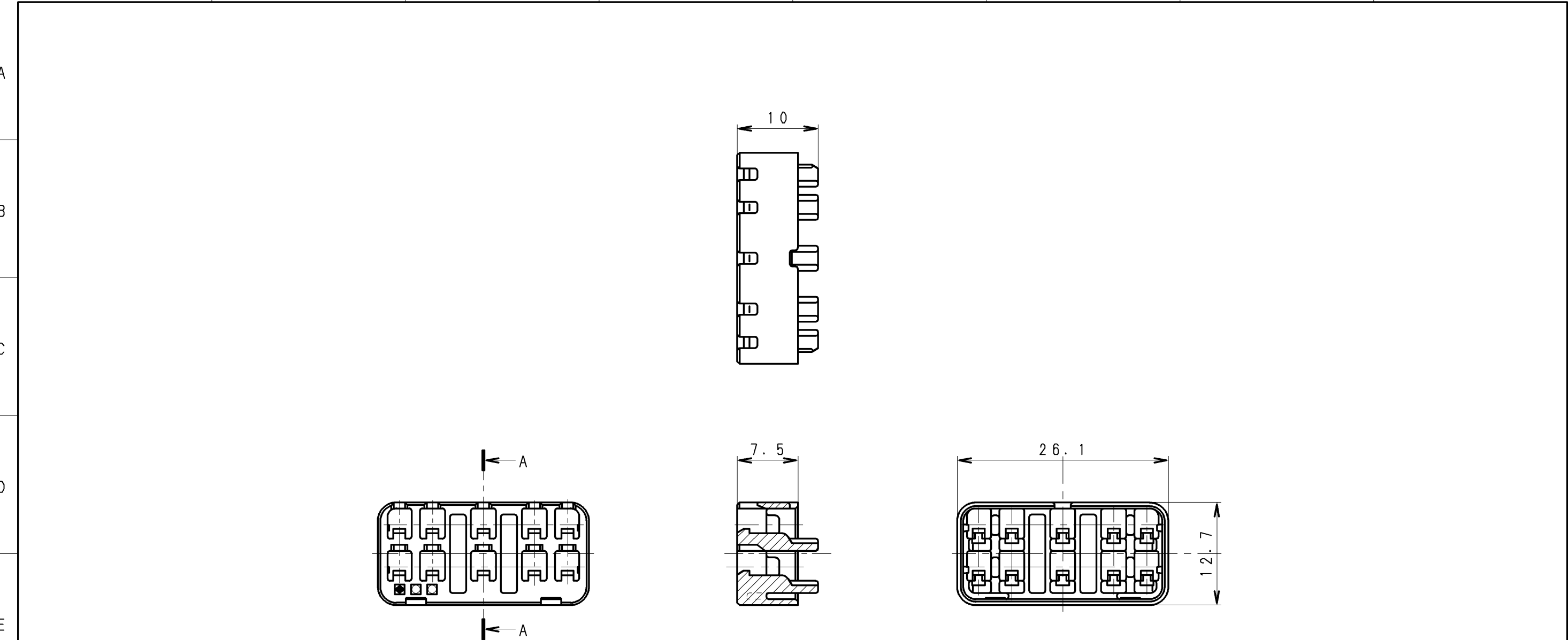
SECTION AA
