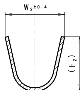
SEC. B-B
