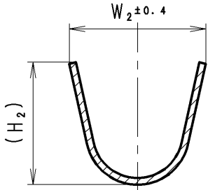
SEC. B-B
