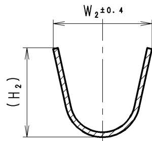
SEC. B-B
