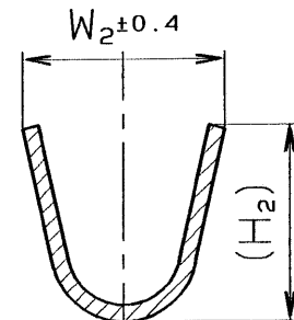
SEC. B-B
