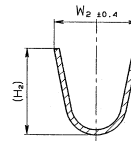
SEC. B-B
