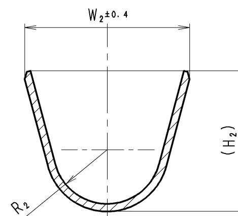
SEC. B- B
