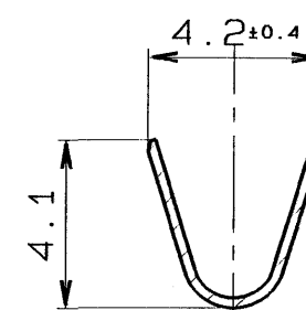
SEC. B-B
