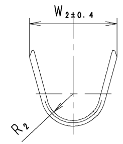
SECTION BB
