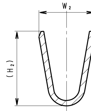
SEC. B-B
