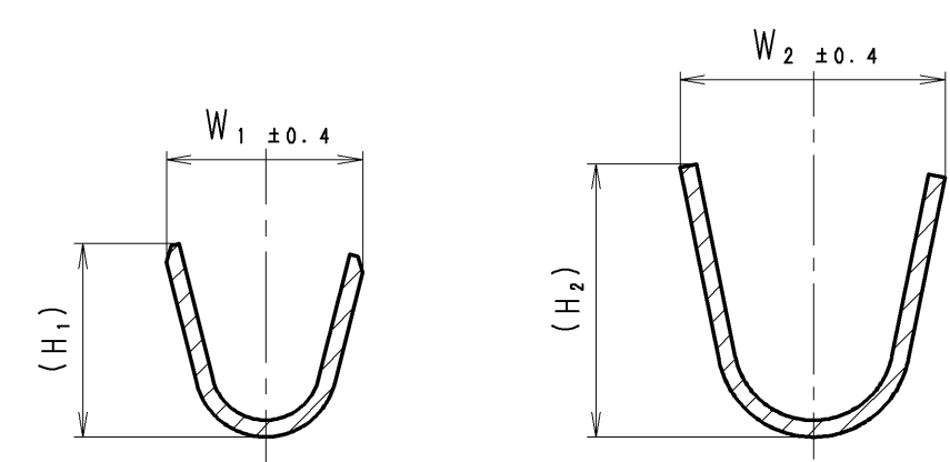
SEC. B- B
