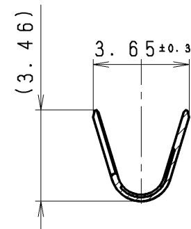
SEC. B-B
