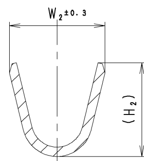
SEC. B-B
