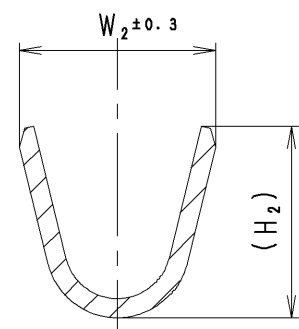
SEC. B-B
