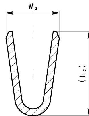
SEC. B-B
