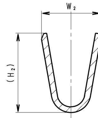
SEC. B-B
