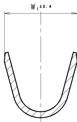
SECTION B-B
