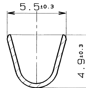
SEC. C-C
