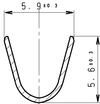
SEC. B-B
