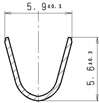
SEC. B-B
