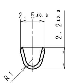
SEC. B-B
