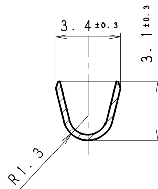
SEC. B- B
