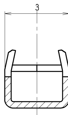
SEC. C- C (10/1)
