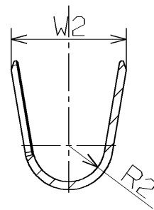
SEC. B-B (SS, SA, S, M SIZE)
