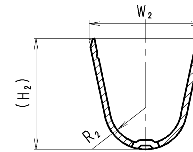
SEC. C-C ( M, L, F SIZE )
