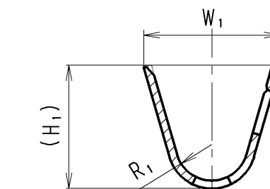
SEC. B- B ( M, L, F SIZE )
