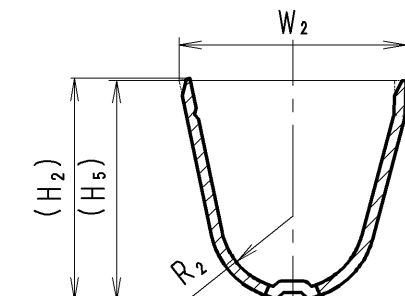
SEC. C-C ( S SIZE )
