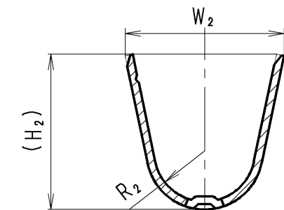
SEC. C-C ( M, L, F SIZE )
