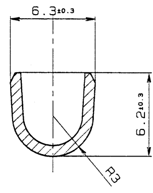
SEC. B-B
