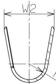
SEC. B-B(SS, S, M SIZE)
