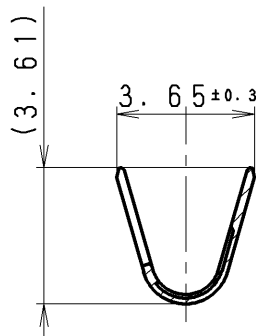
SEC. B-B
