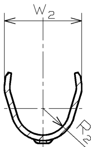
SEC. B-B
