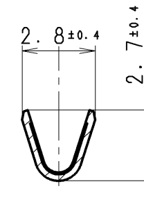
SEC. B-B
