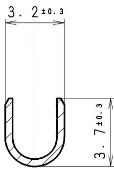
SEC. B-B
