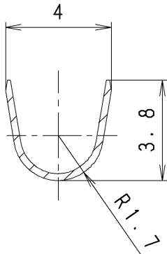
SECTION BB
