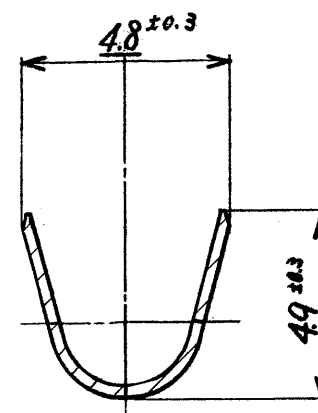
SECTION B-B
