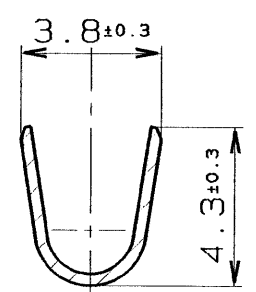
SEC. B-B
