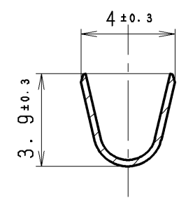
SEC. B-B
